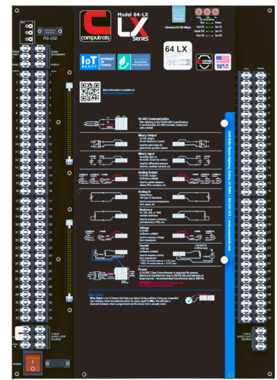
64-LX Controller
