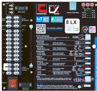
8-LX Controller
