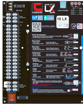
16-LX Controller
